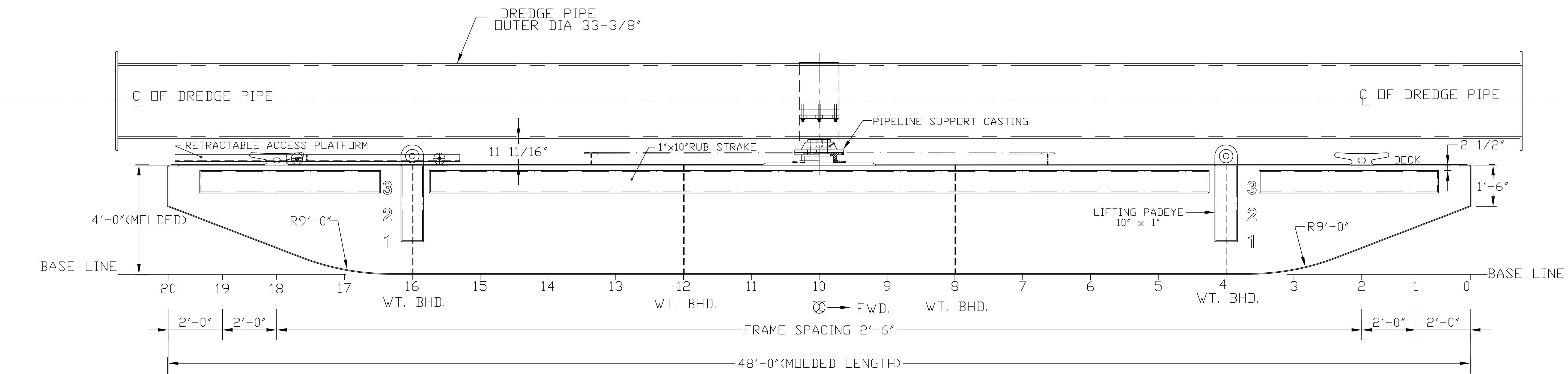
OUTBOARD PROFILE
